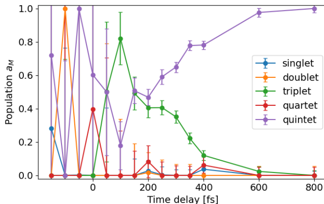
Figure 14: The population curves of the different spin states plotted against the time delay of the optical laser in femtoseconds.
