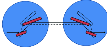
Figure 4: Optical layout of a four-crystal monochromator [?].
