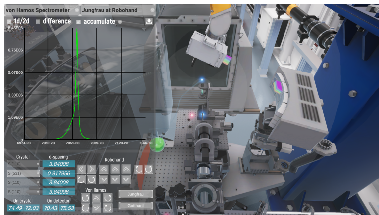
Figure 9: The Von Hamos spectrometer in operating position. with the read-out of the Jungfrau detector as well as the settings for the position to the left.
