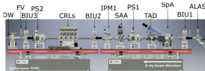
Figure 5: The optical bench in the FXE hut with the following components implemented: BIU 1,2,3 (beam imaging units), SpA (spectrum analyser), TAD (time arrival detector), PS 1,2 (power slits), SAA (solid attenuator assembly), IPM1 (intensity position monitor), CRLs (compound refractive lenses) [4].
