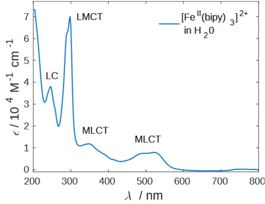
Figure 8: UV/VIS absorption spectrum of an aqueous [\text{Fe}(\text{bipy})_3]\text{Cl}_2 solution. The different CT transitions are indicated. The measured molar absorptivity \epsilon values lie in the expected range of 10^{-4} \text{ l mol}^{-1} \text{ cm}^{-1} to 10^{-5} \text{ l mol}^{-1} \text{ cm}^{-1} for dipole-allowed transitions[4]
