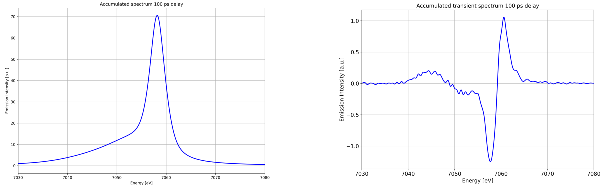
Figure 11: On the left the XES spectrum with the excitation laser on at a delay of 100 ps is plotted. On the right there's the difference spectrum at the same time delay.
