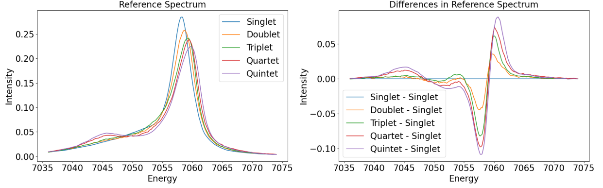
Figure 10: The reference spectra plotted with provided data for different spin states. The reference difference spectra with transient signals plotted with provided data for different transitions.
