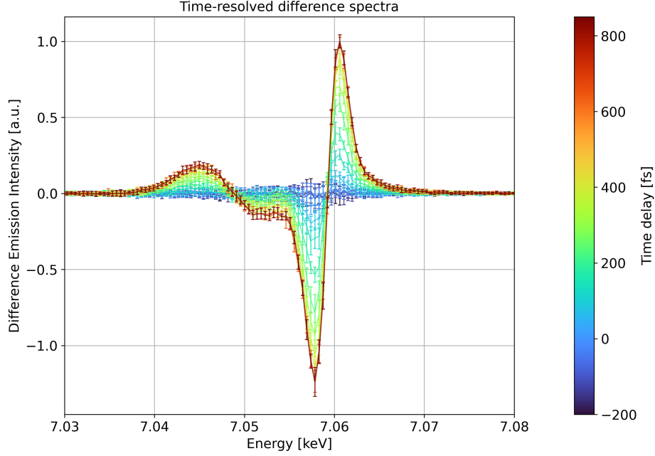
Figure 12: Transient spectra of the X-ray emission at different pump-probe time delays.
