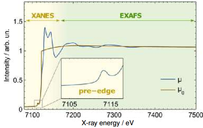
Figure 6: X-Ray absorption spectrum of [\text{Fe}(\text{terpy})_2]^{2+} (terpy: terpyridin) at the Fe K edge displaying the XANES and EXAFS regions including the background absorption contributions \mu_0 . The inset zooms into the weak pre edge features [4].
