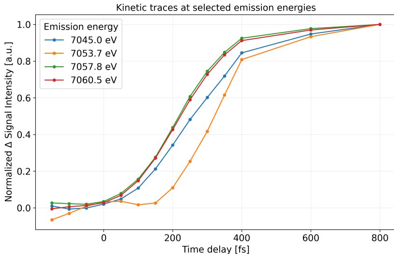
Figure 13: Kinetic traces at selected emission energies.
