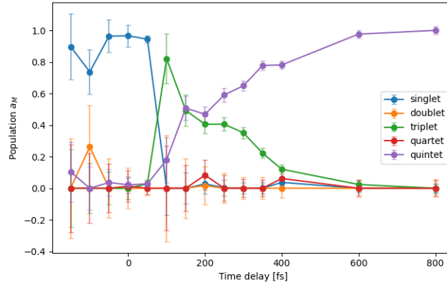
Figure 17: The adjusted population curves of the different spin states plotted against the time delay of the optical laser in femtoseconds.
